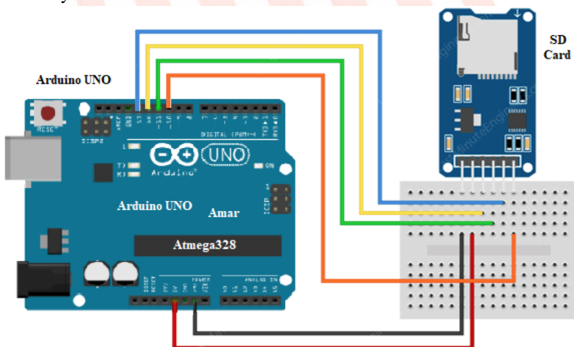
4-rasm. Arduino uno qurilmasiga SD Card ulanishi
