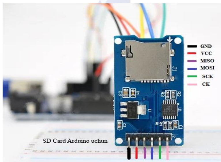
1-rasm. SD Card moduli
