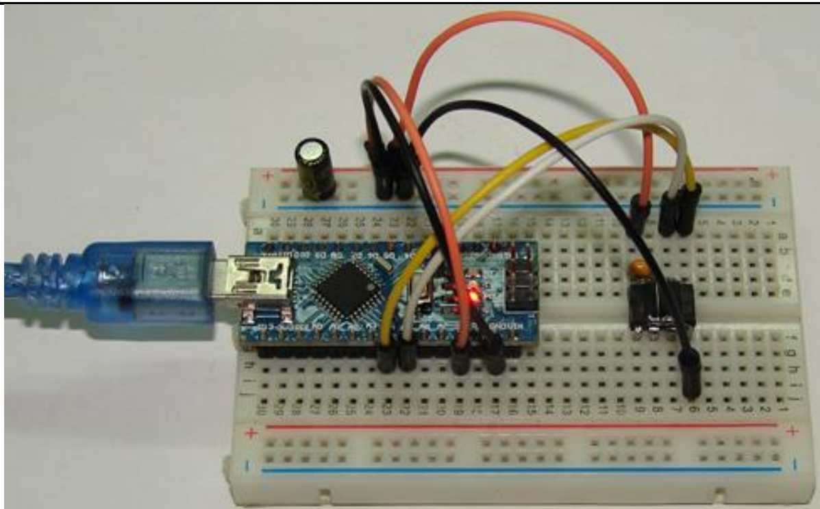
8-rasm. Arduino qurilmasida va EEPROM modulining ulanishi
